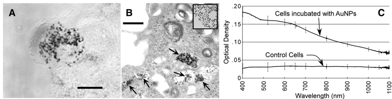
Figure 2. (A) Light micrograph of the in vitro uptake and aggregation of lipoic acid AuNPs in the cytoplasm of one tumor cell. Bar = 10 μm. (B) Higher magnification electron micrograph of a cell after incubation with AuNPs. Aggregation of AuNPs can be seen in the endosomes/lysosomes. Inset at the same magnification shows unaggregated 15 nm AuNPs that exhibit the unaggregated spectrum shown in Figure 1, A. Bar = 500 nm. (C) Spectra of cells incubated with or without AuNPs. Cells incubated with AuNPs showed absorption in the NIR region. Error bars are from 6 separate measurements.
