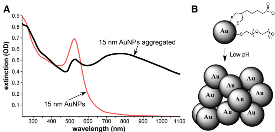
Figure 1. (A) Change in spectra of 15 nm AuNPs before (red) and after (black) aggregation, here induced by lowering the pH to 5 in 150 mM NaCl. A large increase in the near infrared absorbance (750–1000 nm) is evident. (B) Aggregation of AuNPs at low pH. AuNPs coated with lipoic acid and PEG show aggregation at the pH of endosomes and lysosomes. Gold core size of the AuNPs was measured to be 15.3 \pm 1.0 nm by electron microscopy and the hydrodynamic diameter in solution was measured to be 21.6 \pm 0.1 by dynamic light scattering. The thiol ligands are not removed upon aggregation (here reversible with pH), but are not shown in the aggregated clump for clarity.
